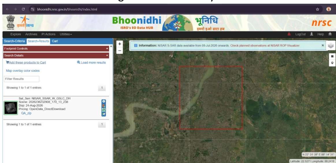
Figure 6.6: NISAR S-SAR Product Search Result in Bhoonidhi Portal
