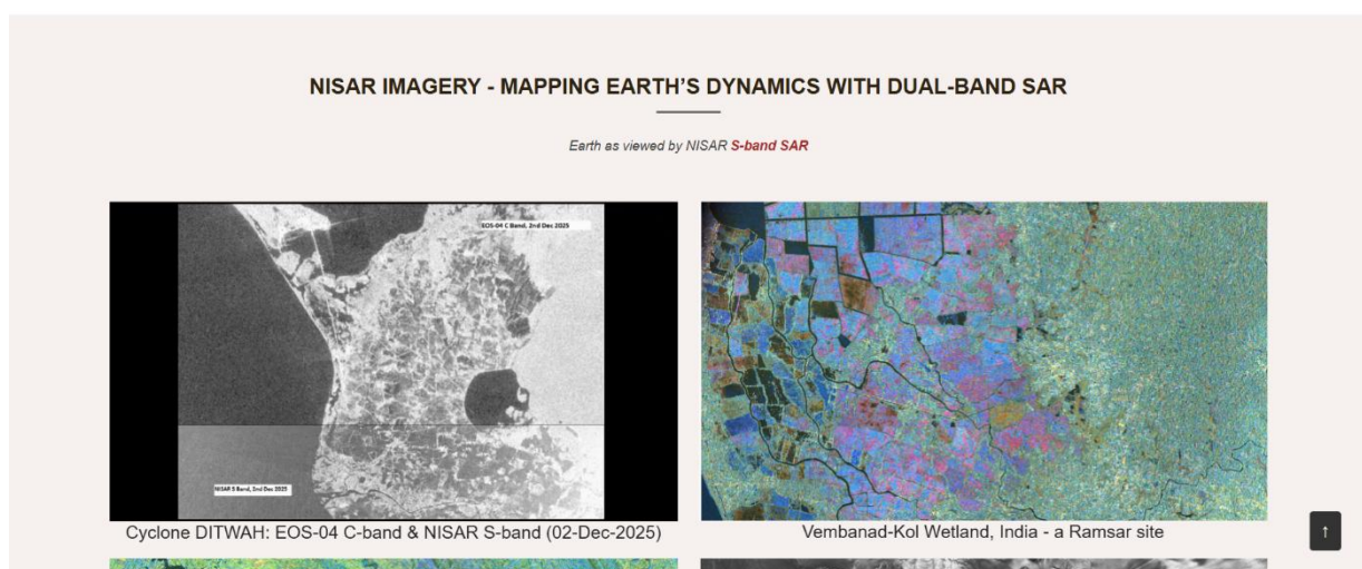
Figure 7.1: Examples of NISAR S-band SAR Applications in Earth Observation
